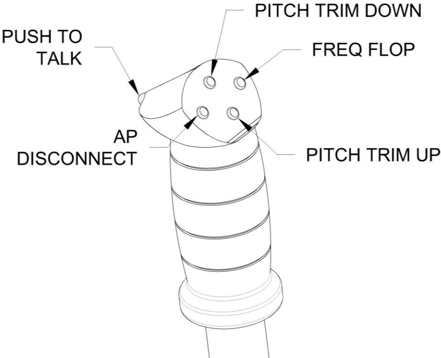
FIGURE 7-6 STICK SWITCHES
