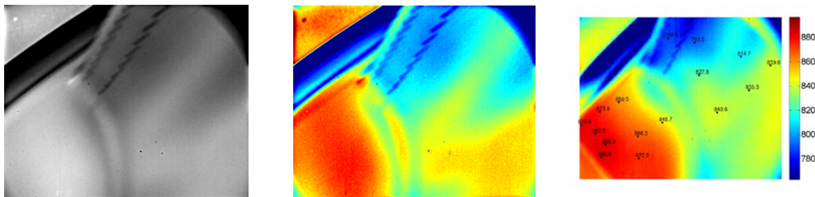
Figure 5: Compressor turbine blade 1, full speed test September 2012.
