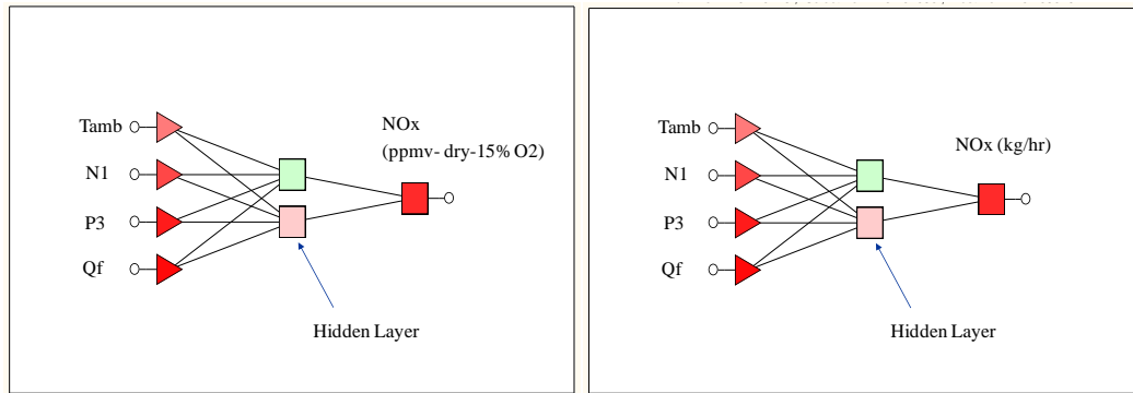
Figure 3: MLP Architecture for NO x Prediction.
