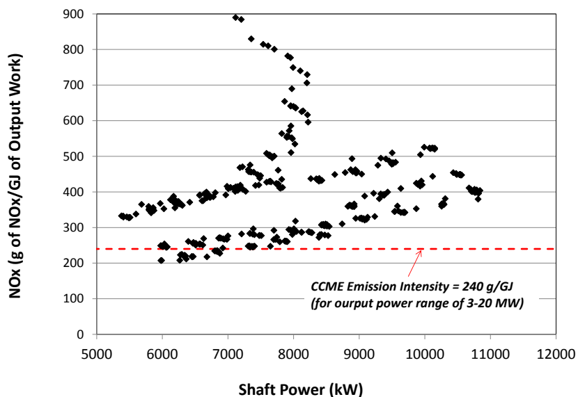
Figure 8b: Measured Emission Factor and Comparison with 1992 CCME Emission Intensity.
