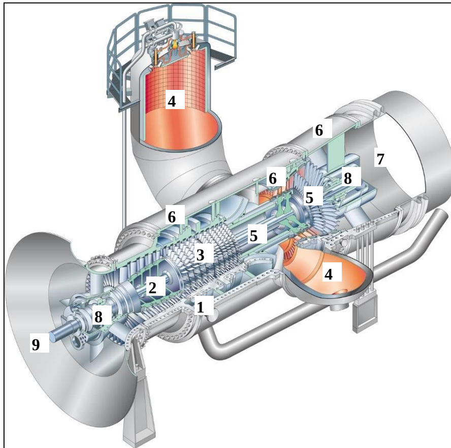
Figure 2: SGT-2000E Design
