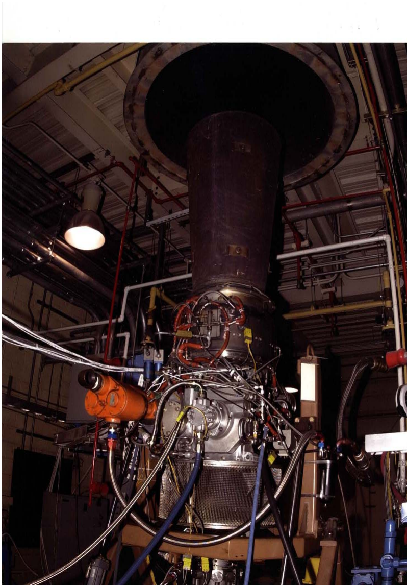
Figure 4. ASE40V Demonstration Test Apparatus
