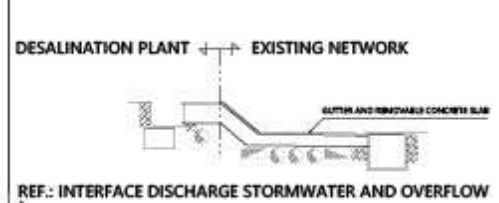
REF.: INTERFACE DISCHARGE STORMWATER AND OVERFLOW
