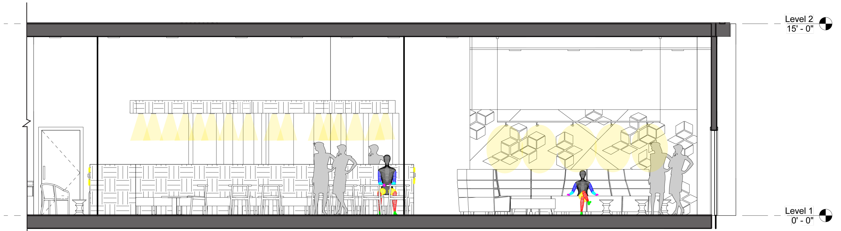
TRANSVERSE SECTION
