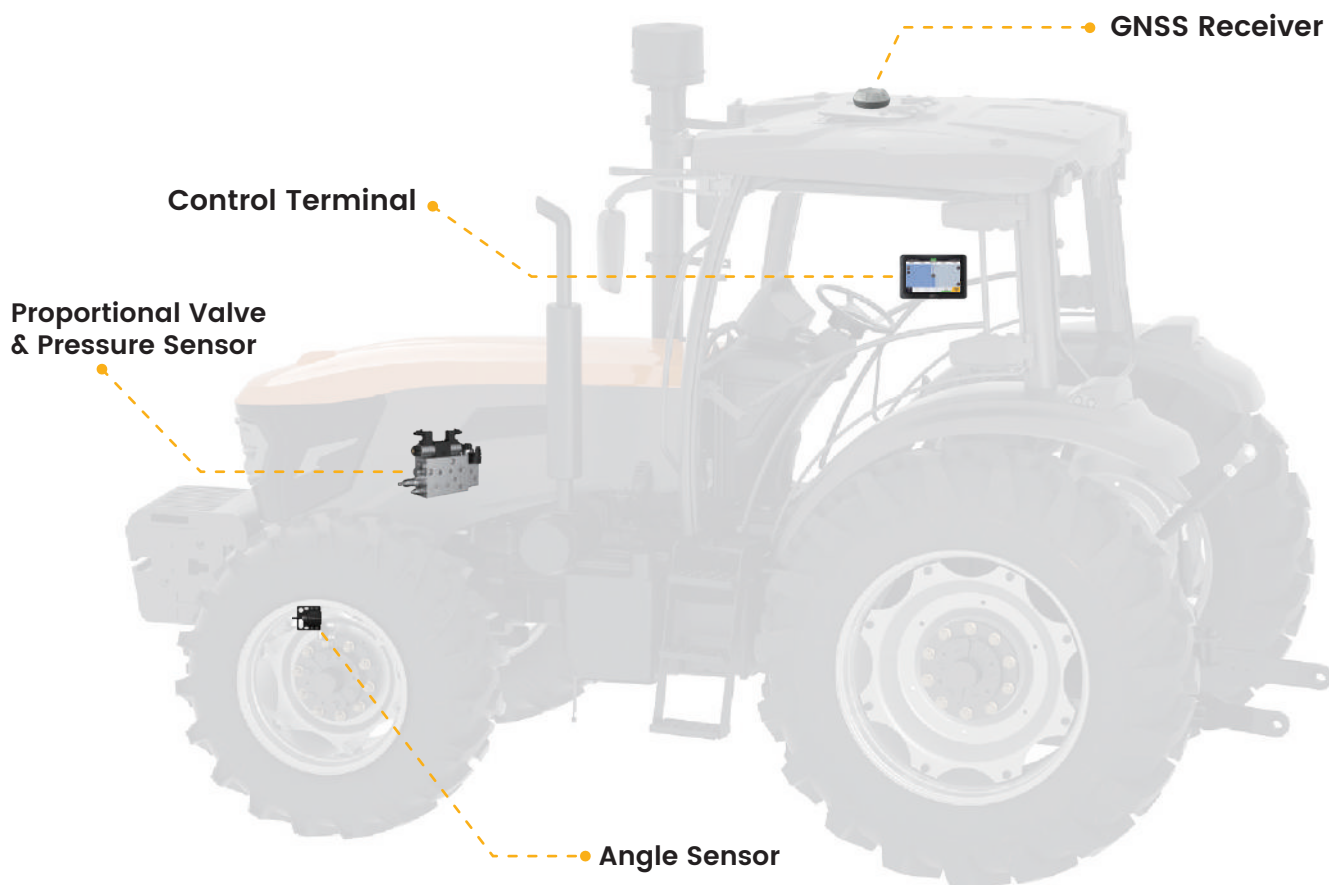
Angle Sensor
