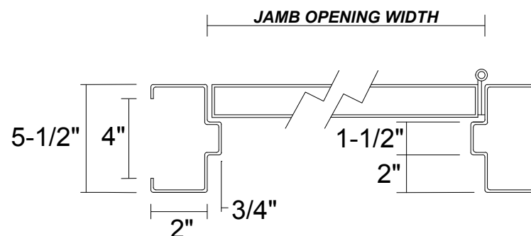
PLAN VIEW
