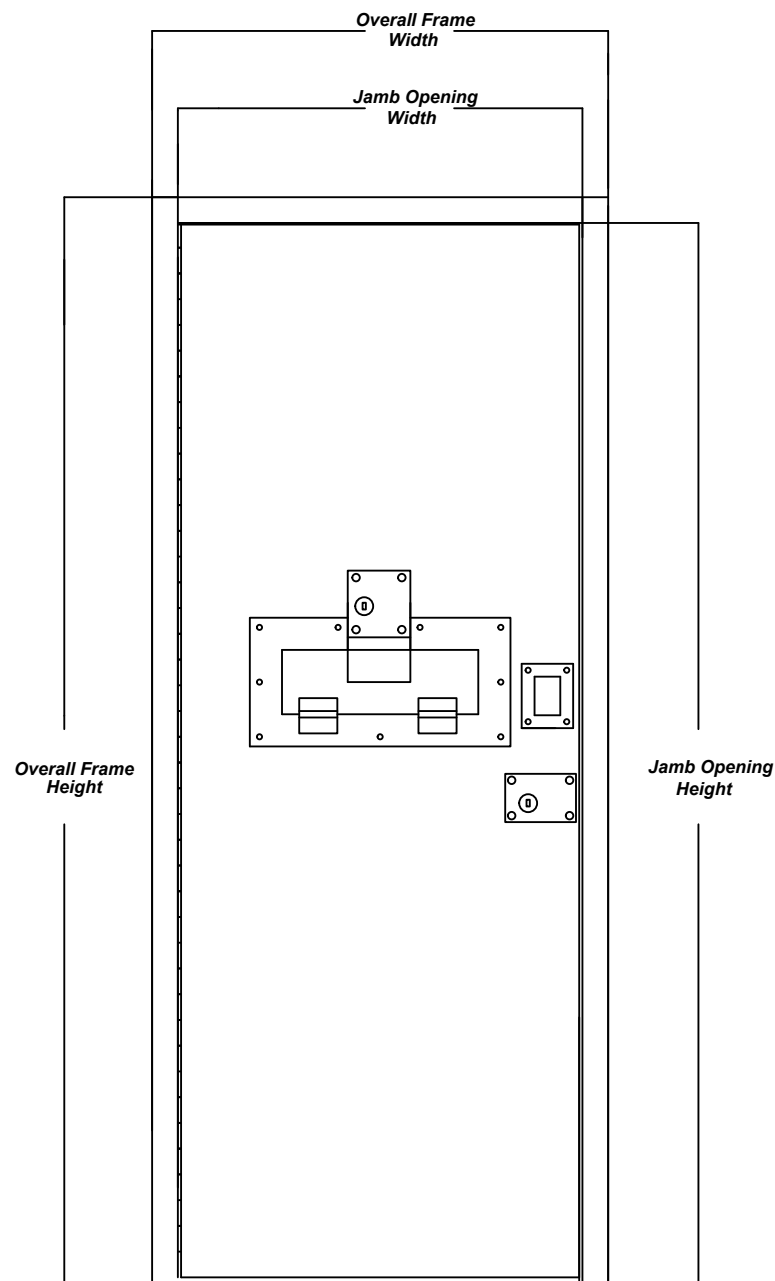
THREAT SIDE ELEVATION
