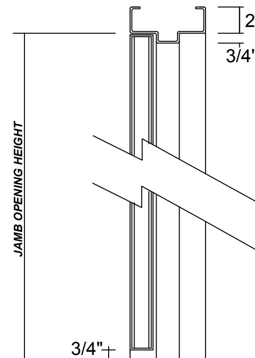
SECTION VIEW
