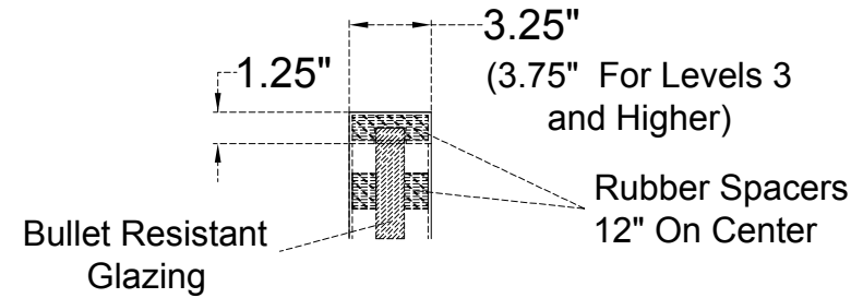
HEAD/JAMB SECTION
