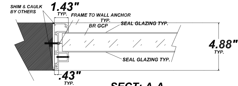
SECT: A-A
