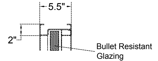
HEAD/JAMB/SILL SECTION
