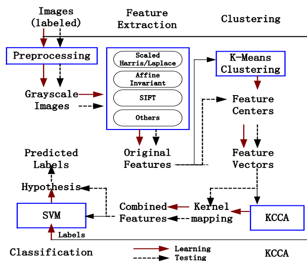
Figure 1. The proposed system framework for generic object recognition
