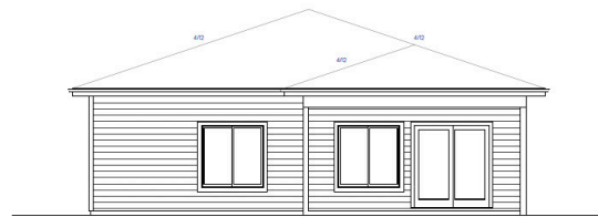
REAR ELEVATION SCALE 1/4"=1'
