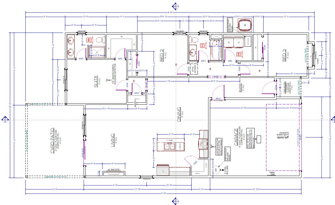
MAIN FLOOR SCALE 1/8"=1'-0" (DOOR LINO. TOP OF WINDOWS & AFF. LINO.)
