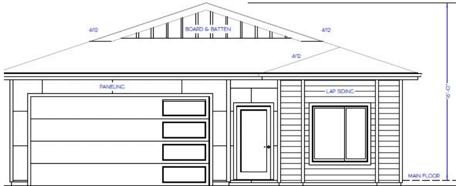
FRONT ELEVATION SCALE 1/4"=1'
