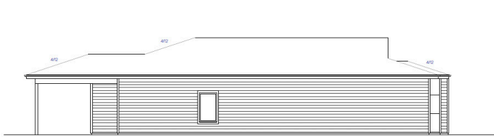
LEFT ELEVATION SCALE 3/16"=1'
