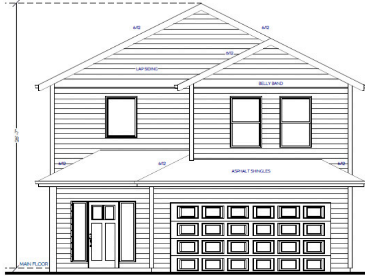
FRONT ELEVATION SCALE 1/4"=1'
