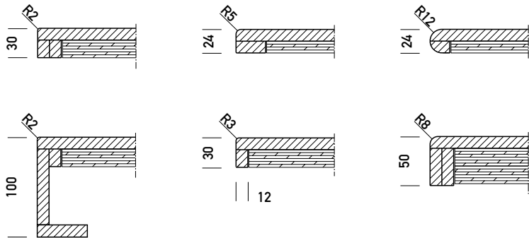
Examples of edge profiles
