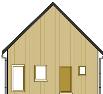
North Elevation
