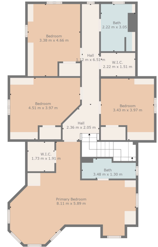
Floor 3
