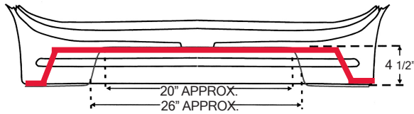
749100 49-52 CHEVY FIREWALL (4 1/2" SET-BACK) 26" Wide
