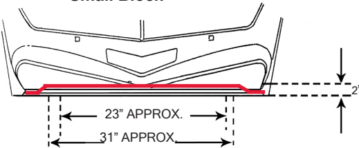
737105 1937-39 CHEVY FIREWALL (2" SET-BACK) Small Block
