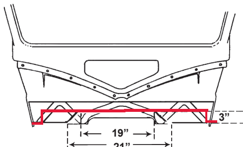
1935-36 Ford Truck Firewall 3" Set-back No 351000
