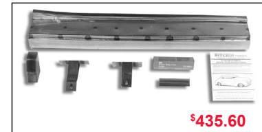
742152 41-48 ROCKER PANEL KIT Front - LH
