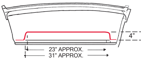
281000 1928-29 FORD FIREWALL (4" Set-Back)
