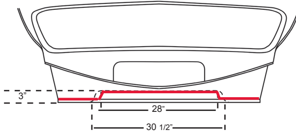
481000 48-52 TRUCK FIREWALL
