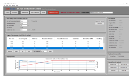
GC×GC Modulation Control Software Method-based PC control interface
