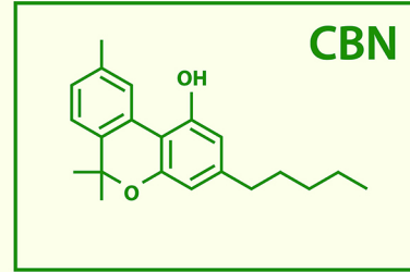
Cannabinol
