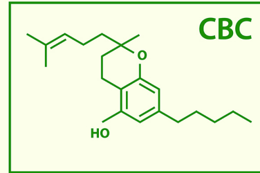
Cannabichromene
