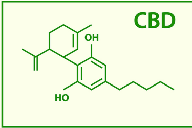
Cannabidiol
