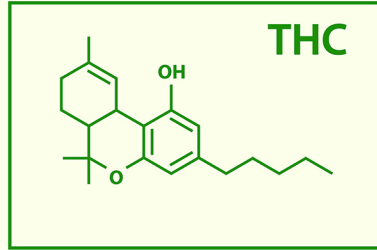
Tetrahydrocannabinol
