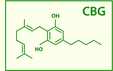
Cannabigerol
