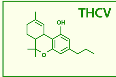
Tetrahydrocannabivarin
