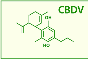
Cannabidivarin
