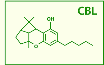
Cannabicyclol
