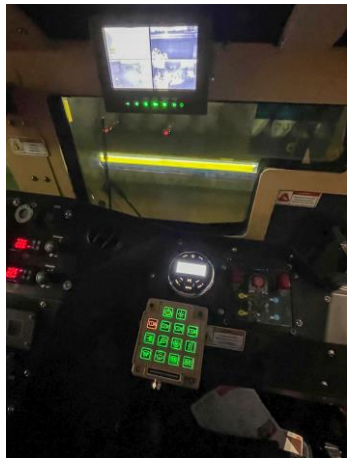
Quad display enables safe driving with defense hatch closed
