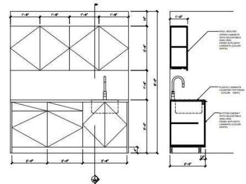
3 KITCHENETTE SECTION SCALE: 3/8" = 1'-0"
