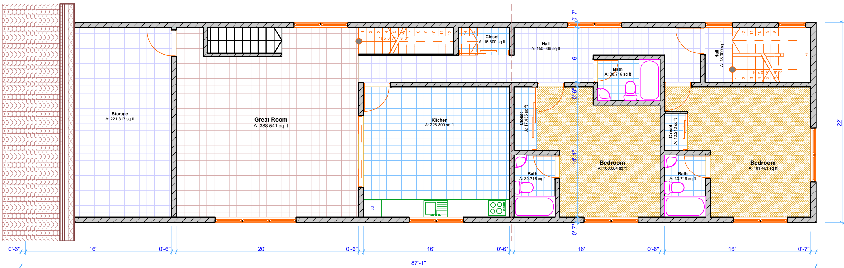
E01-01 - Level 5
