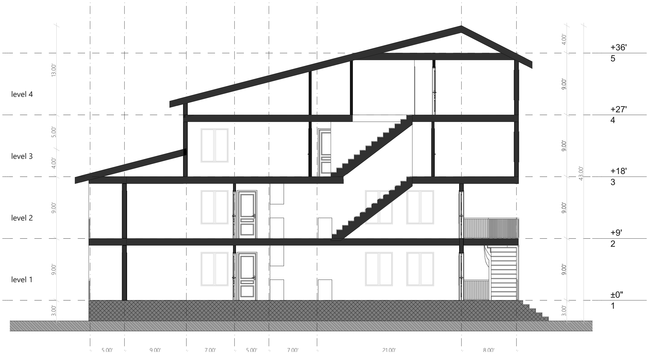
ENERGY 1-02S SECTION 1 SCALE 1: 100
