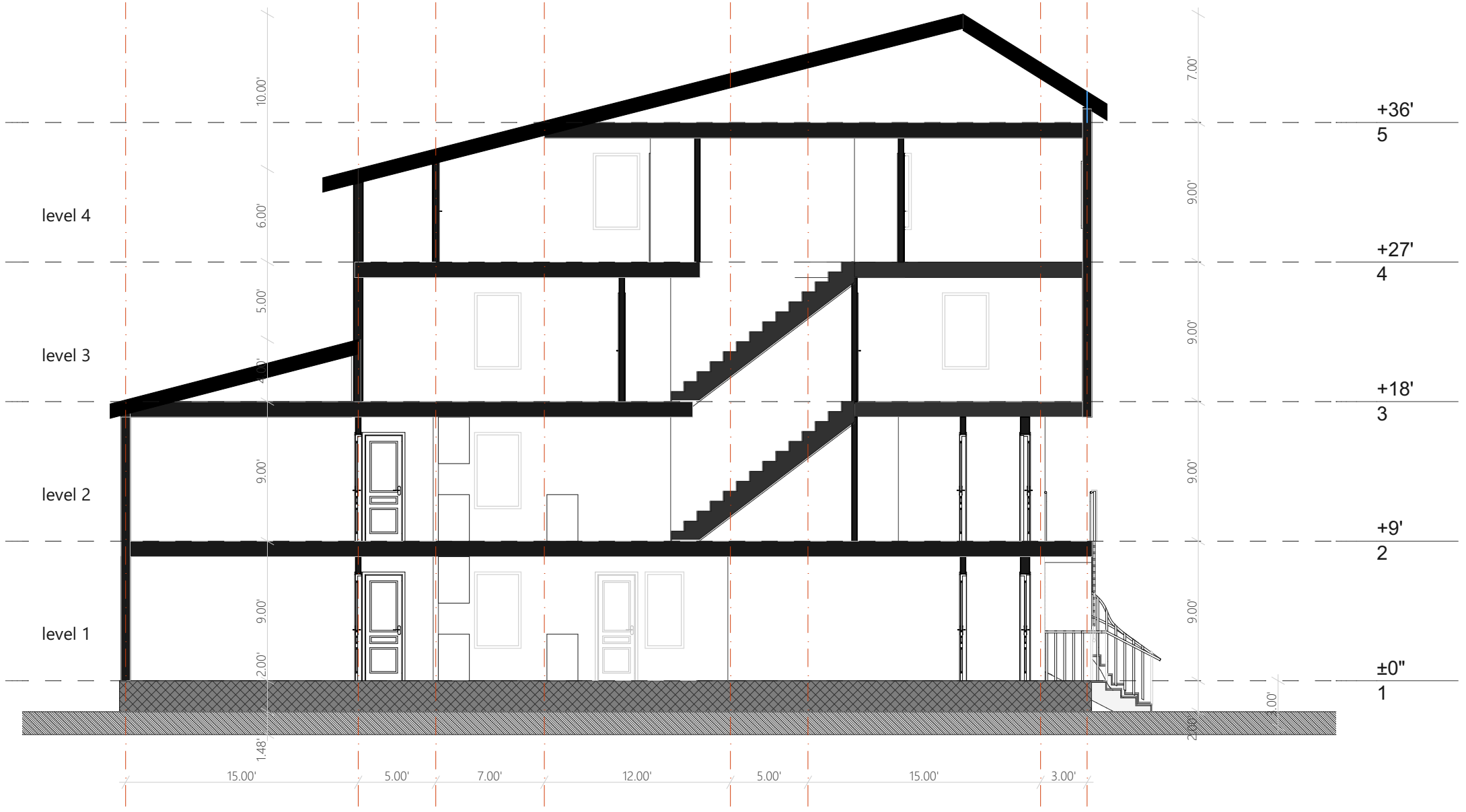
ENERGY 1-RB SECTION 1 SCALE 1: 100
