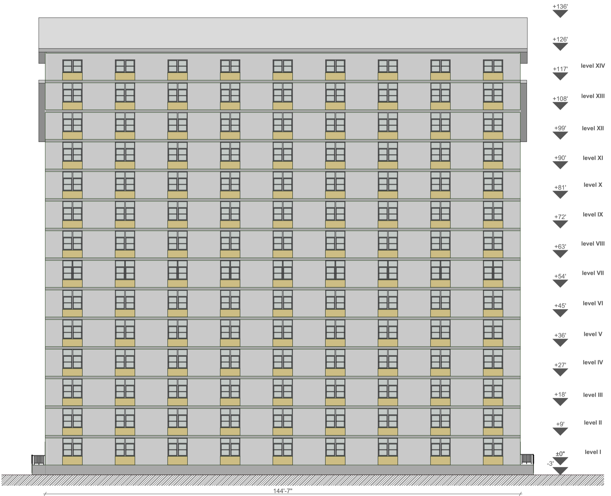
H05-05S NORTH scale 1:200
