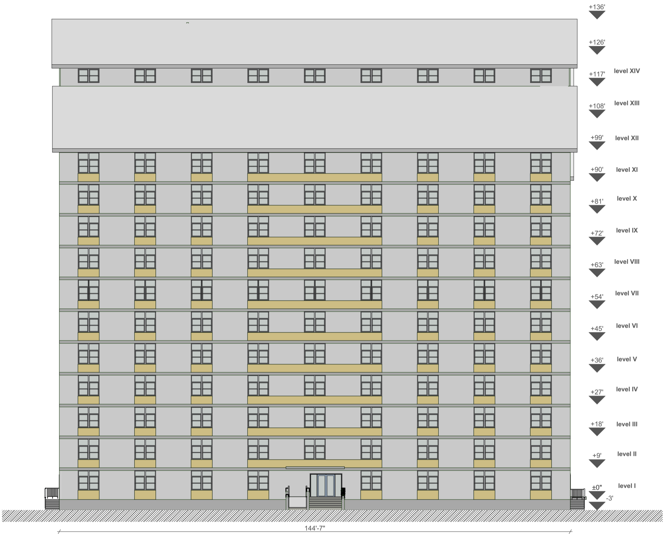
H05-05S SOUTH scale 1:200
