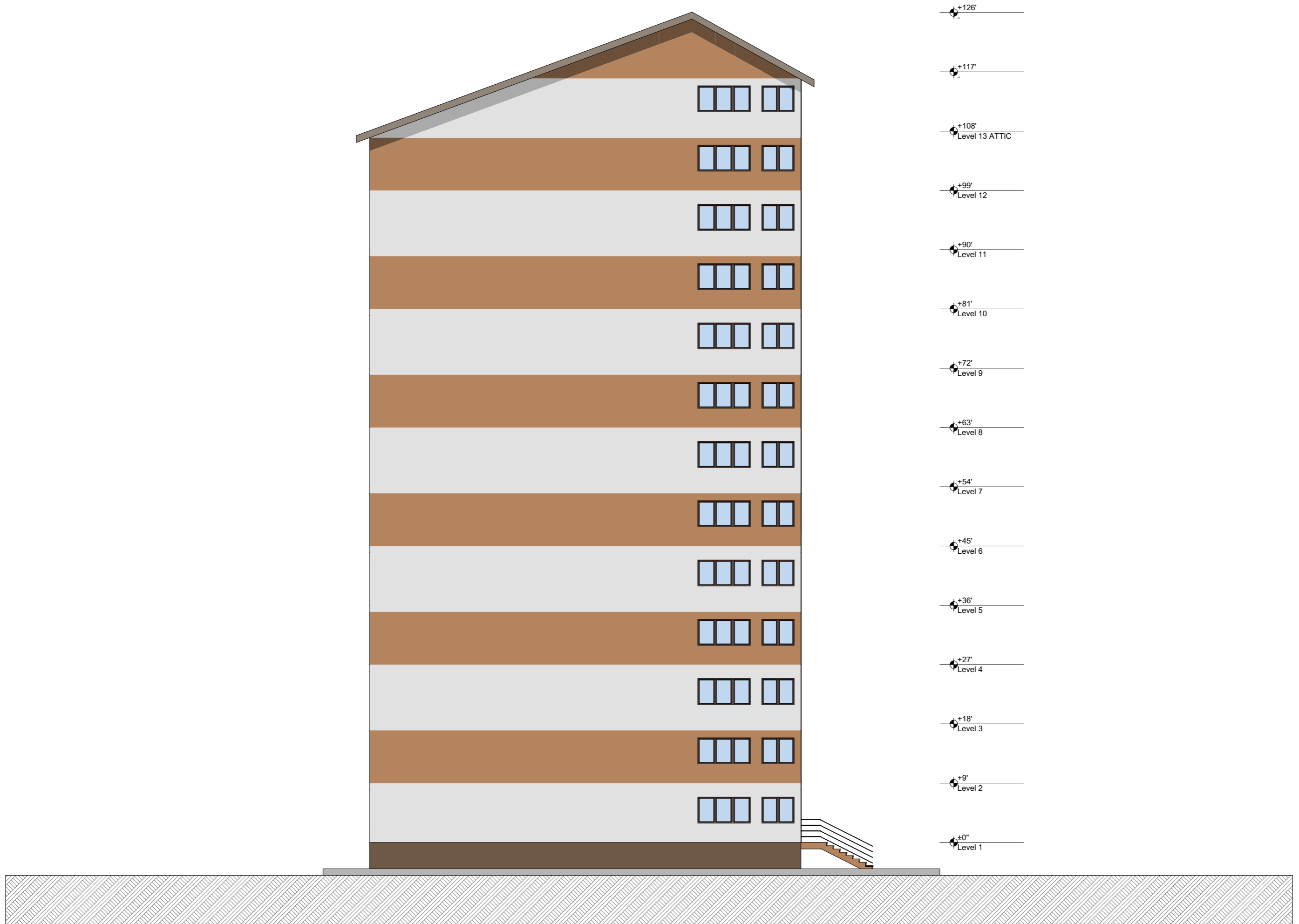
H05-07 - EAST Elevation
