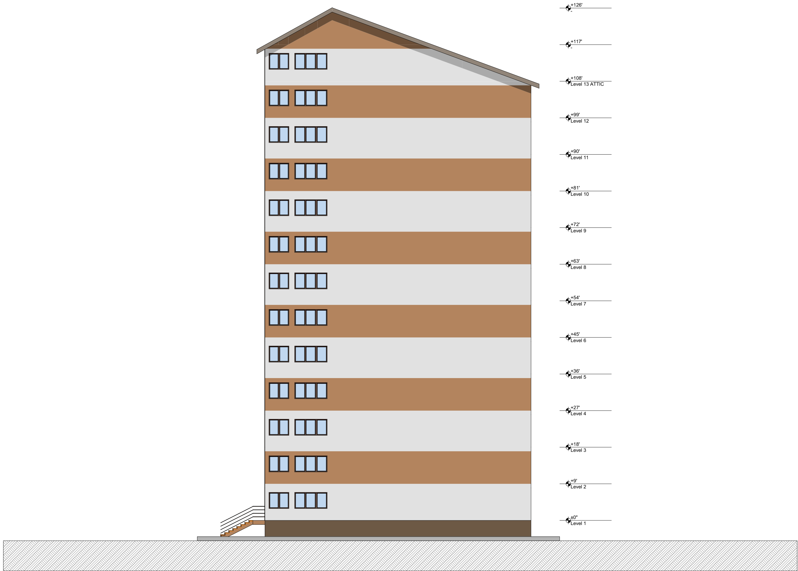
H05-07 - WEST Elevation
