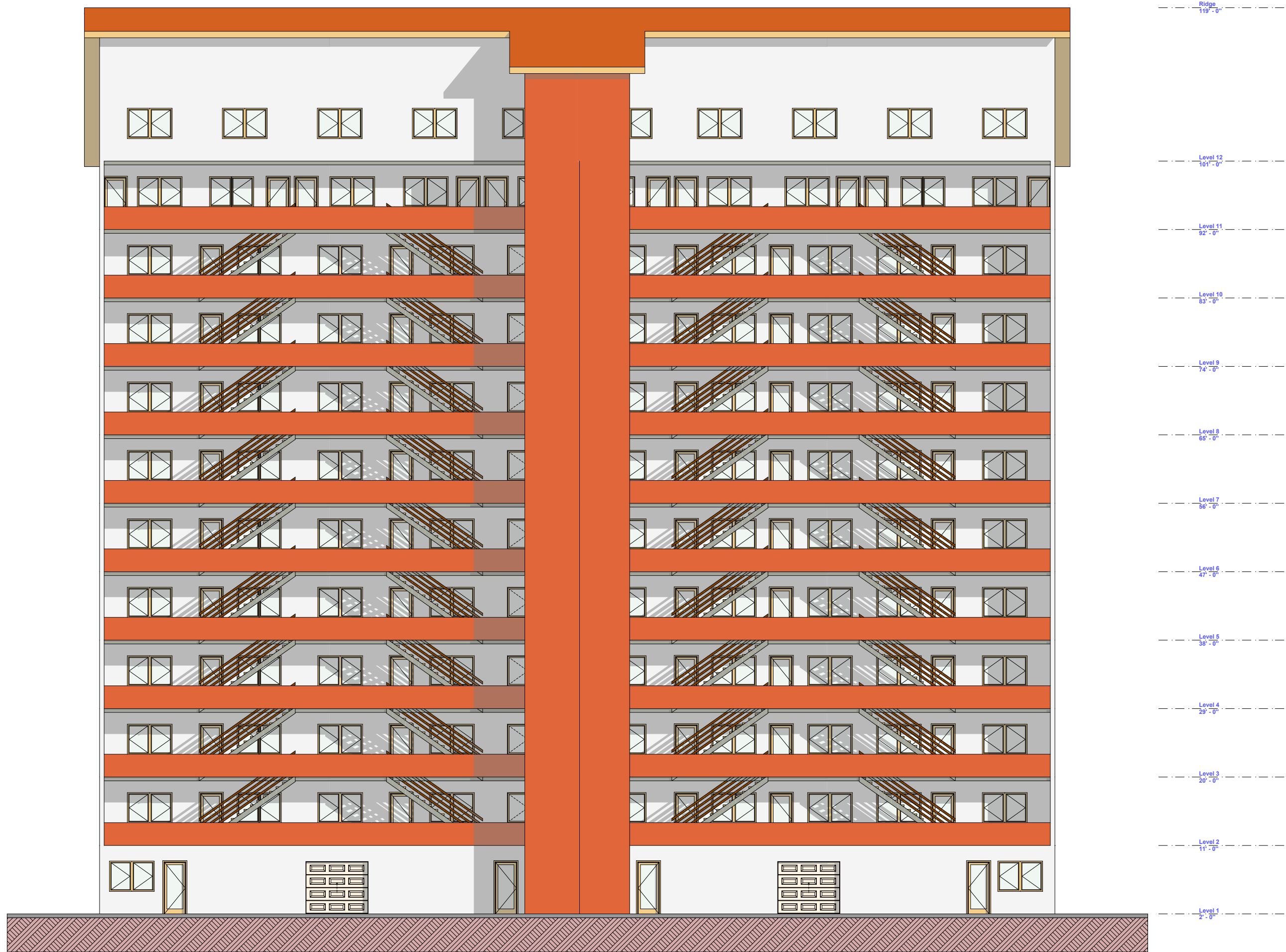
H05-04 - NORTH Elevation
