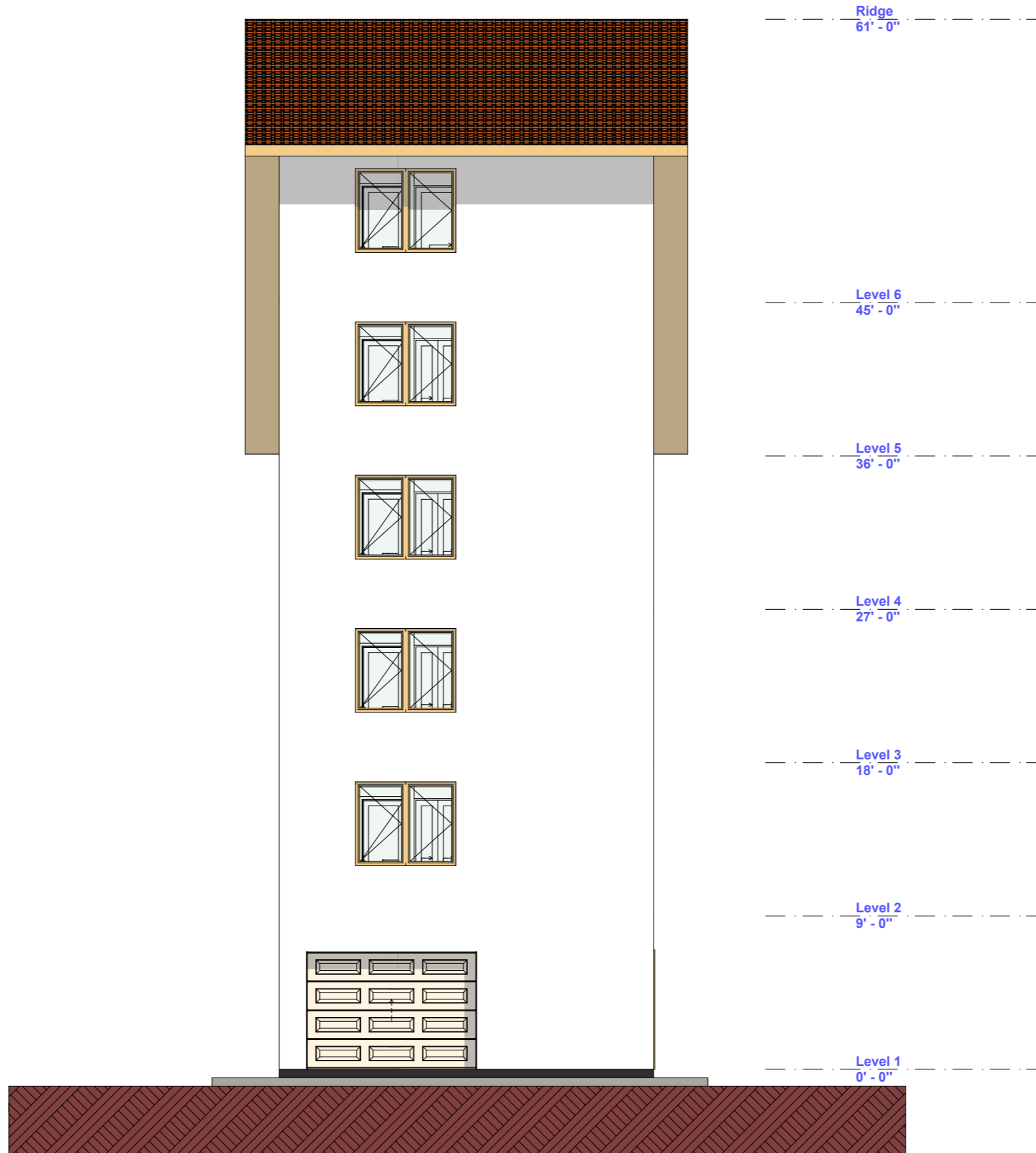
E01-01 North Elevation
