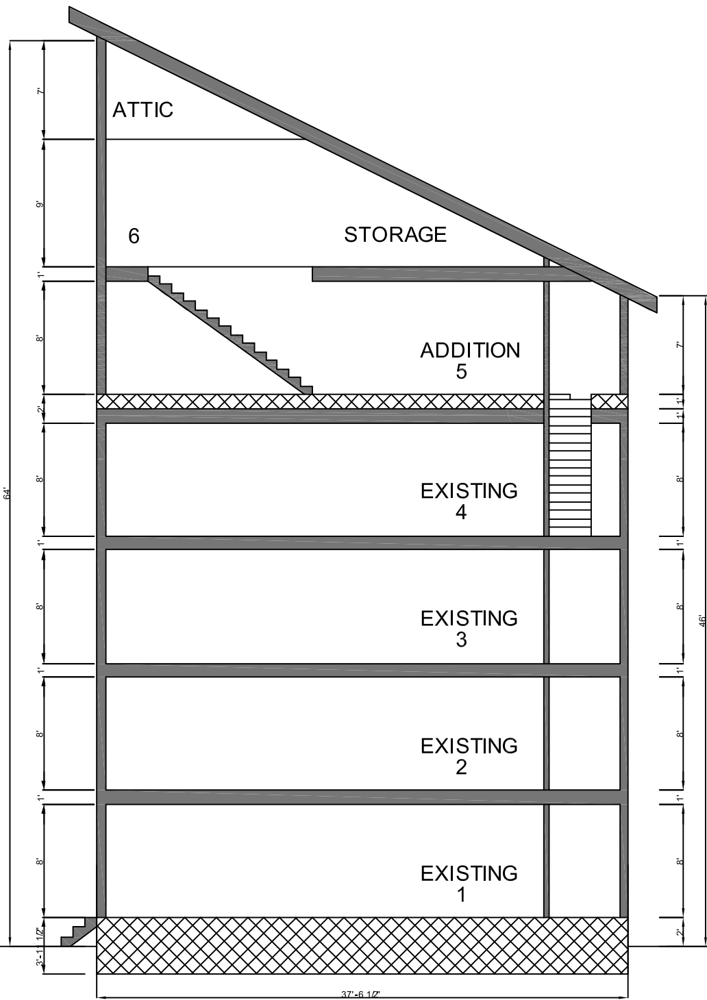
SECTION WEST
