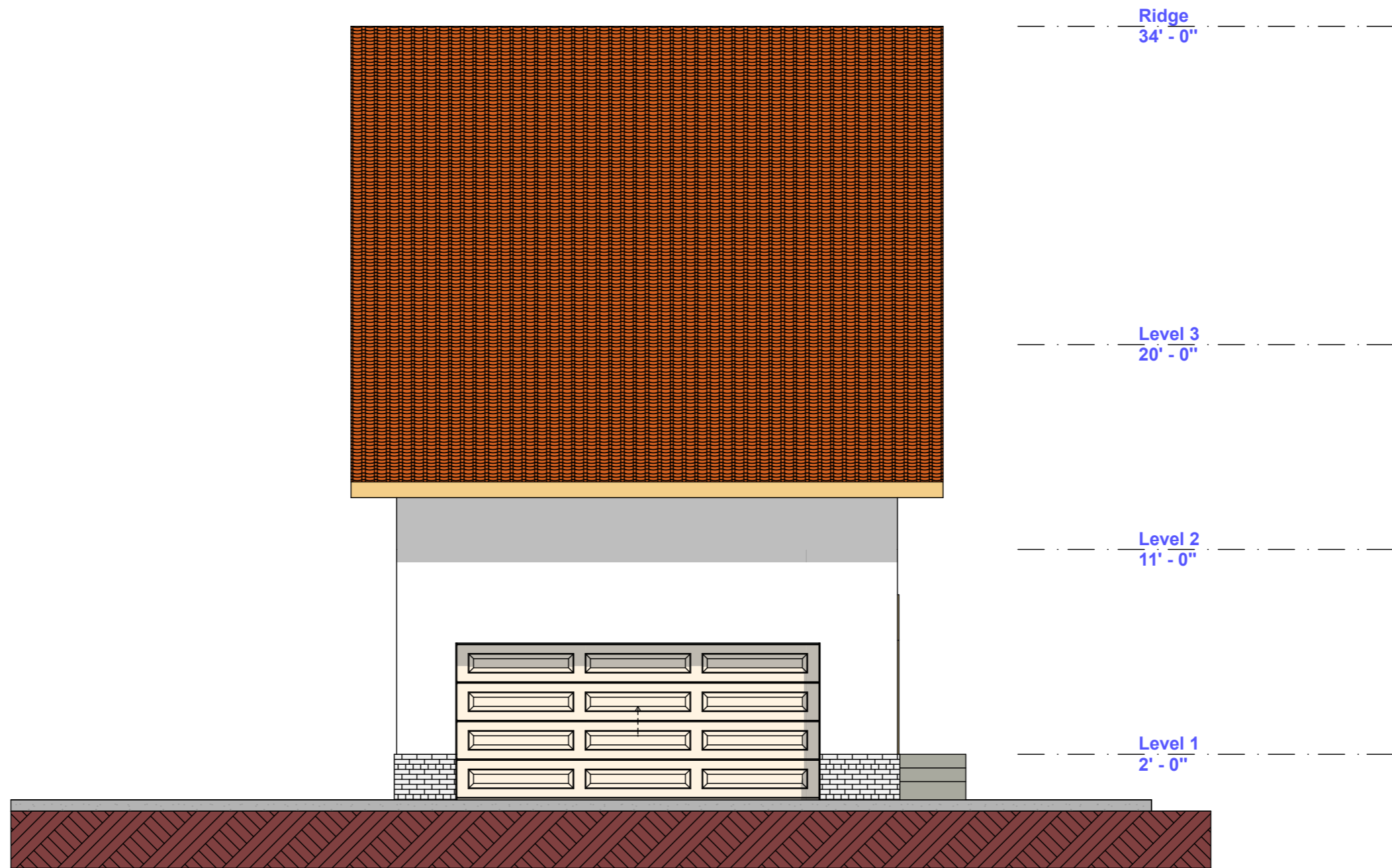
E01-00 SOUTH Elevation
