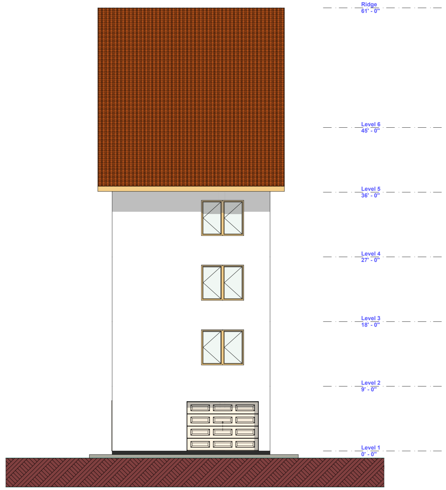
E01-01 South Elevation
