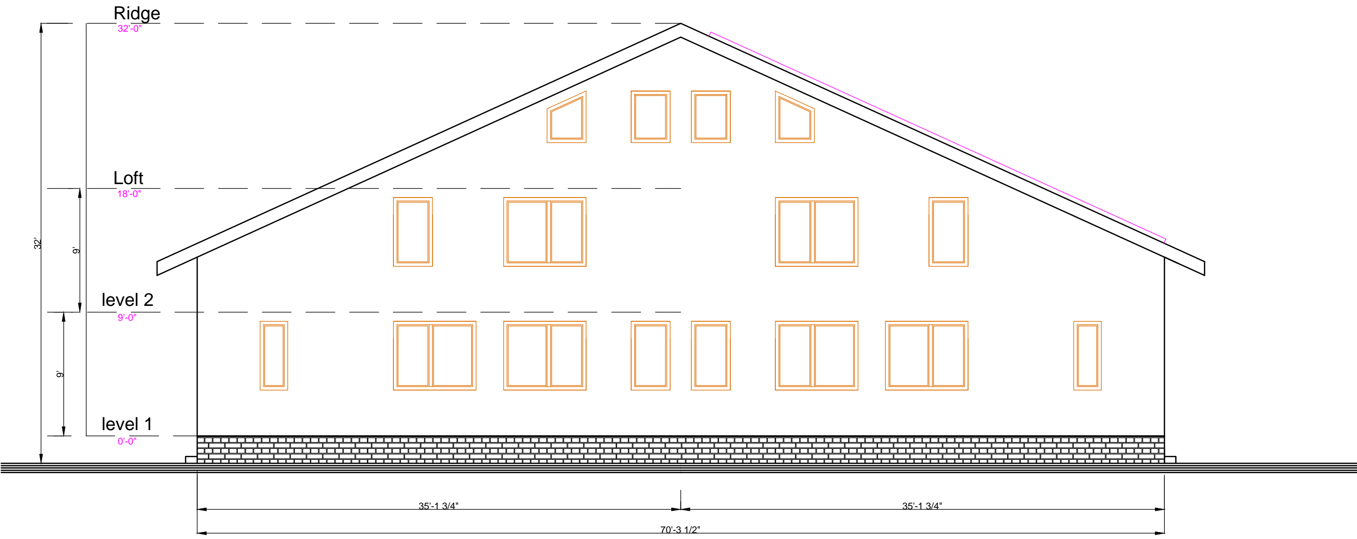
WEST ELEVATION
