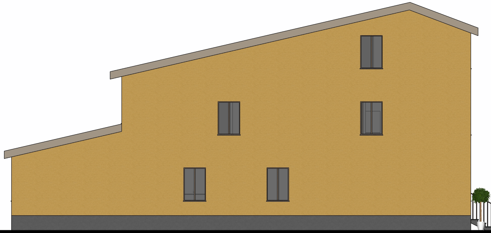
EAST ELEVATION
