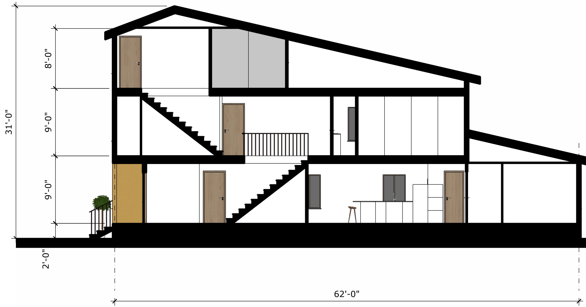
SECTION 1-1
