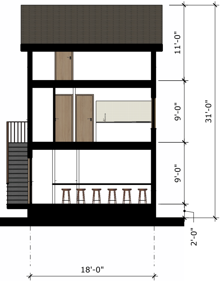
SECTION 2-2
