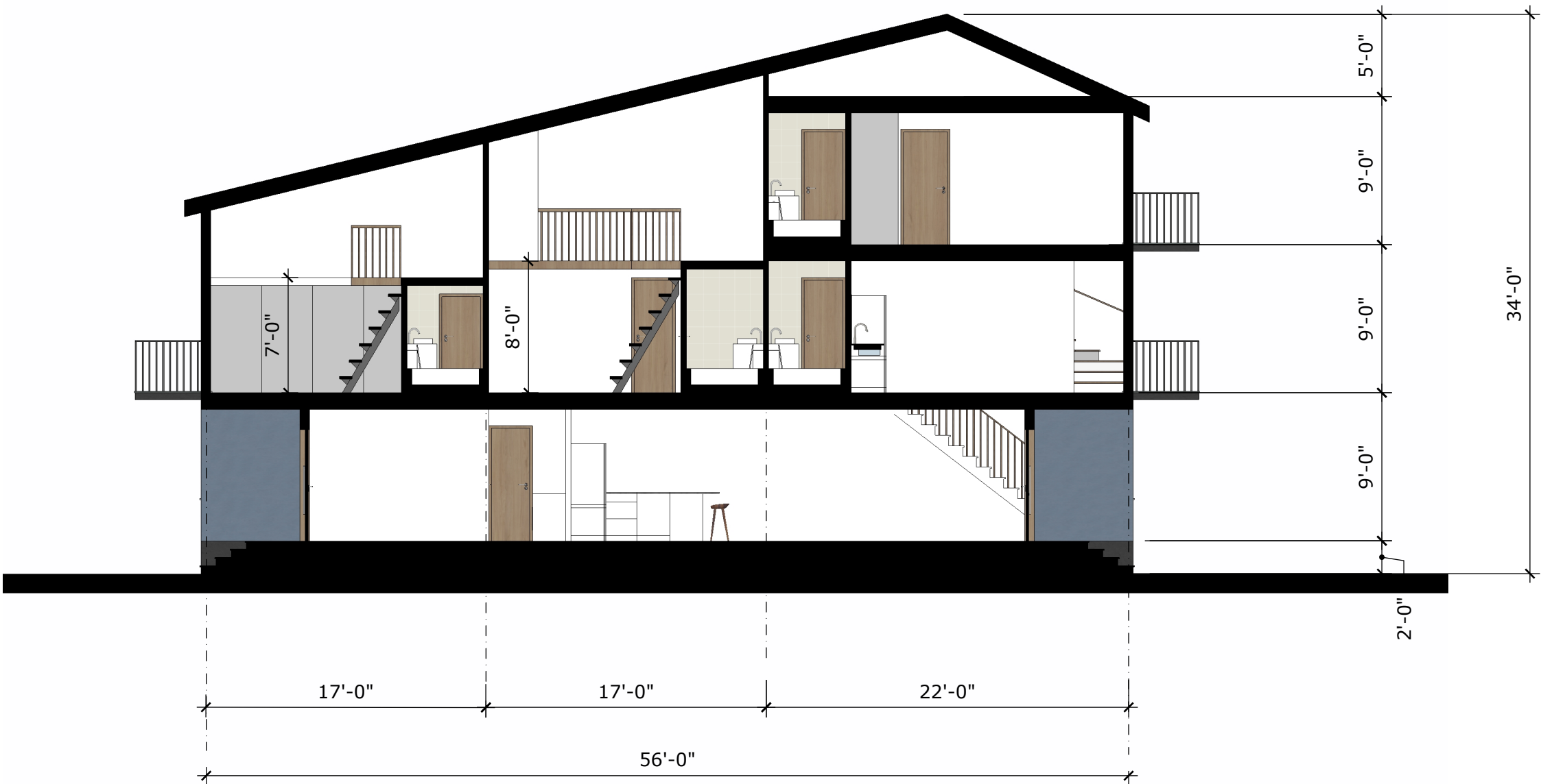
SECTION 1-1
