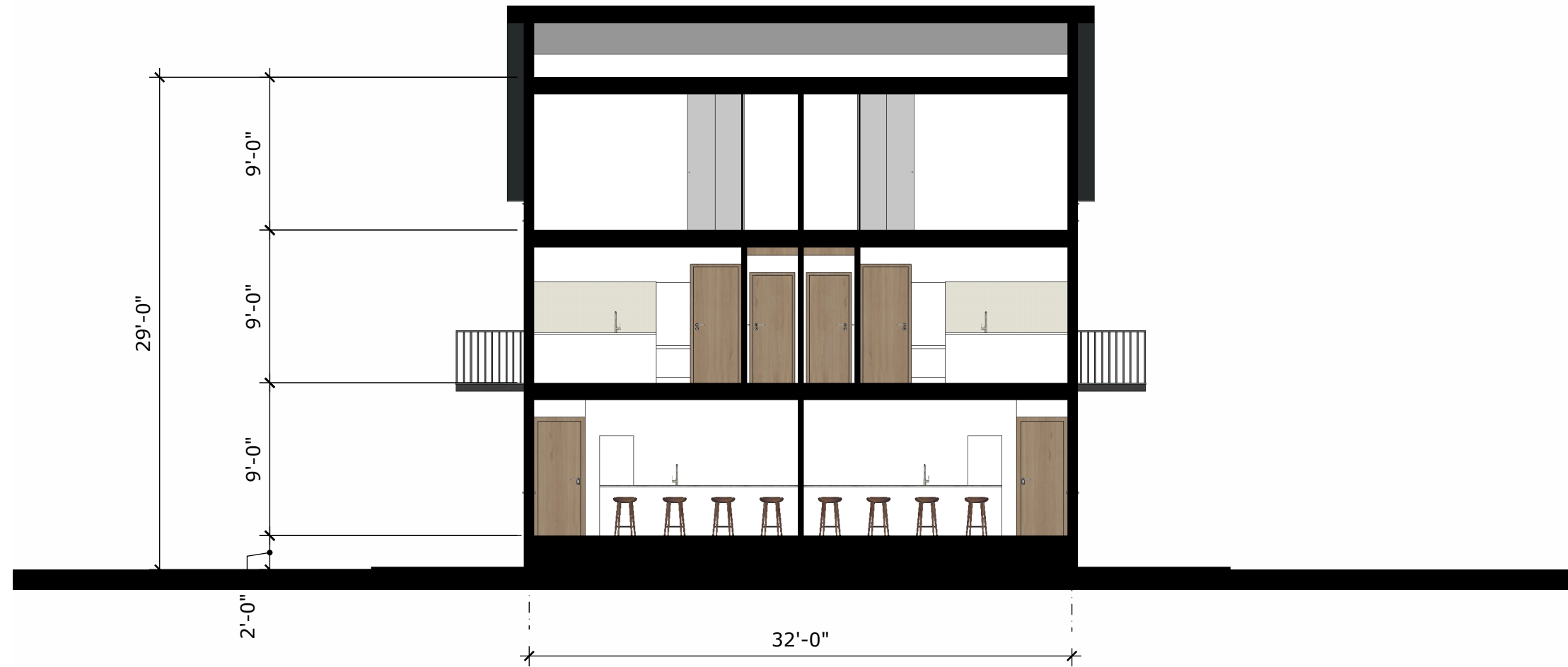
SECTION 2-2
