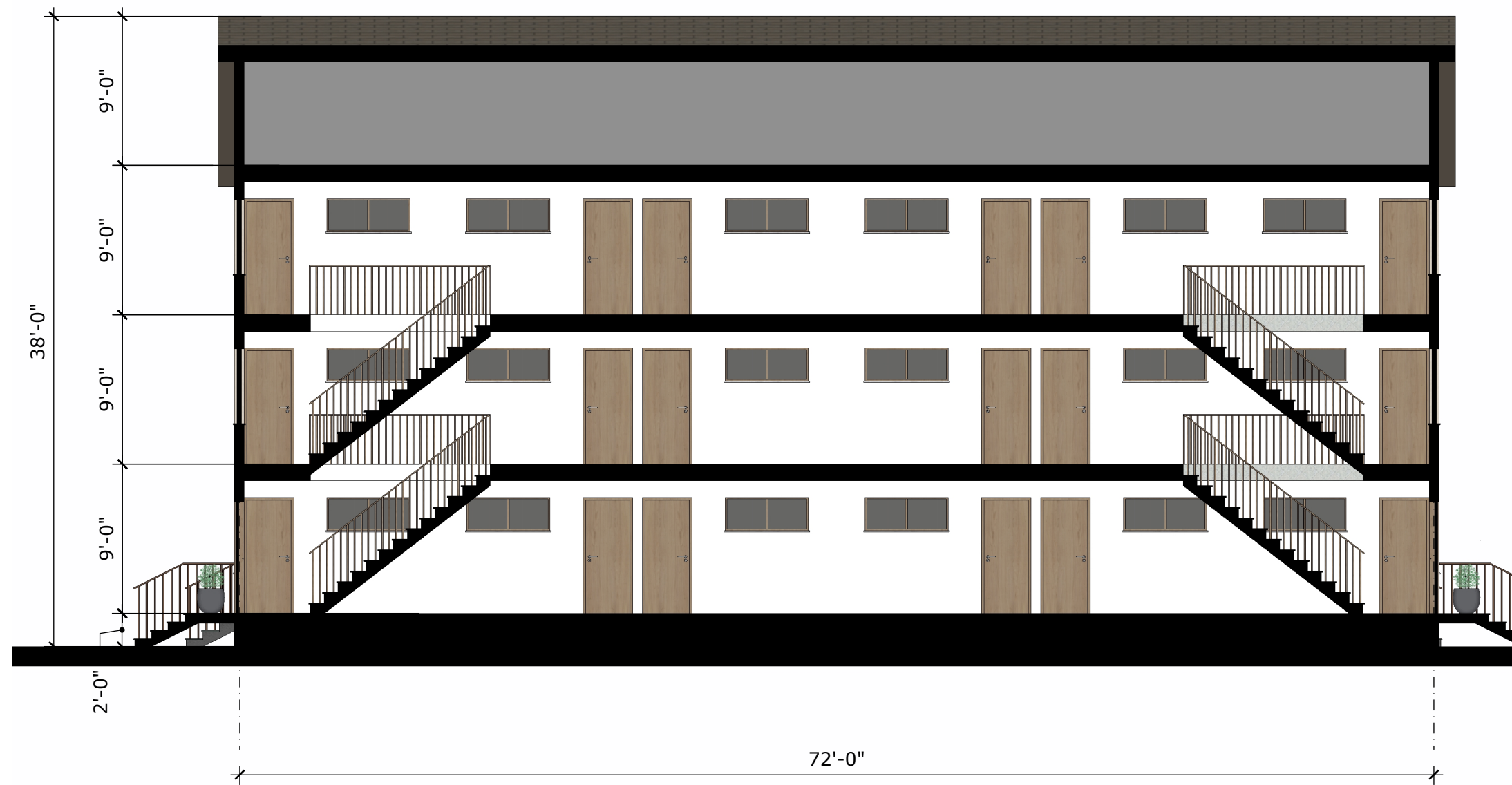
SECTION 1-1
