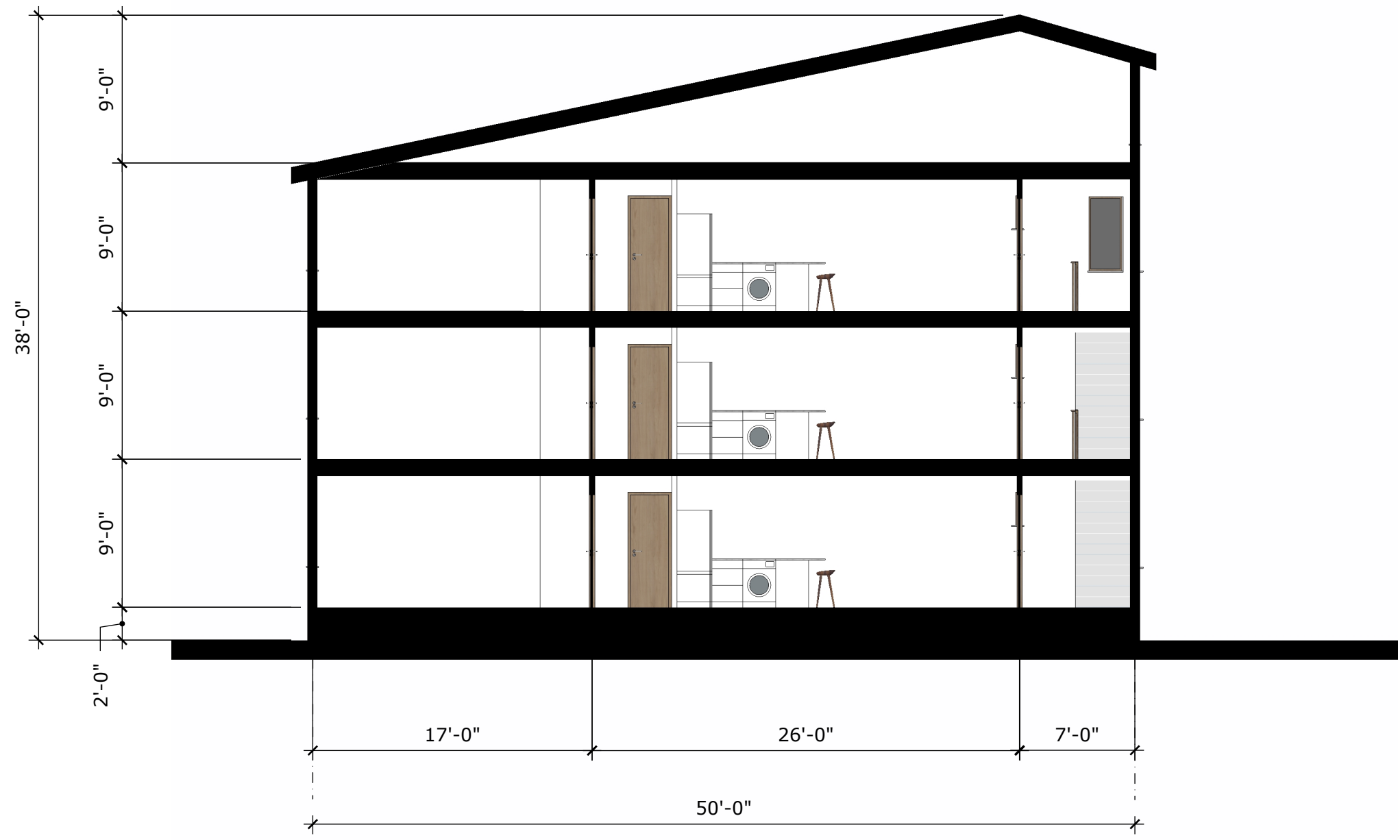
SECTION 2-2
