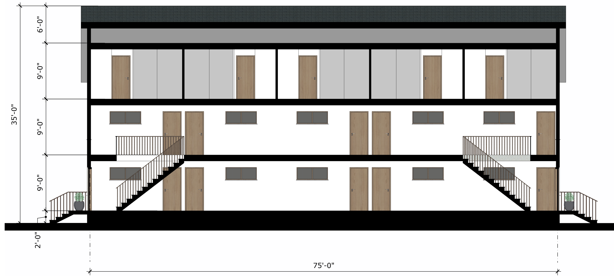
SECTION 1-1
