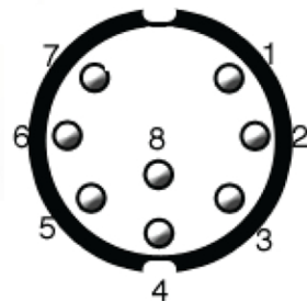
CONXALL Connector and pins (Male connector) View from BACK of plug.
