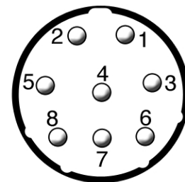
AMP Connector and pins (Male connector) View from back of plug
